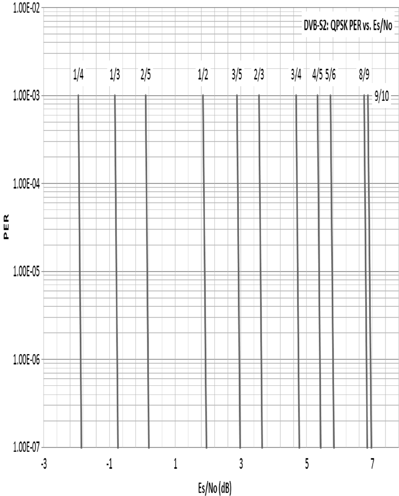
Figure B-1. DVB-S2 QPSK Packet Error Rate versus Es/No
