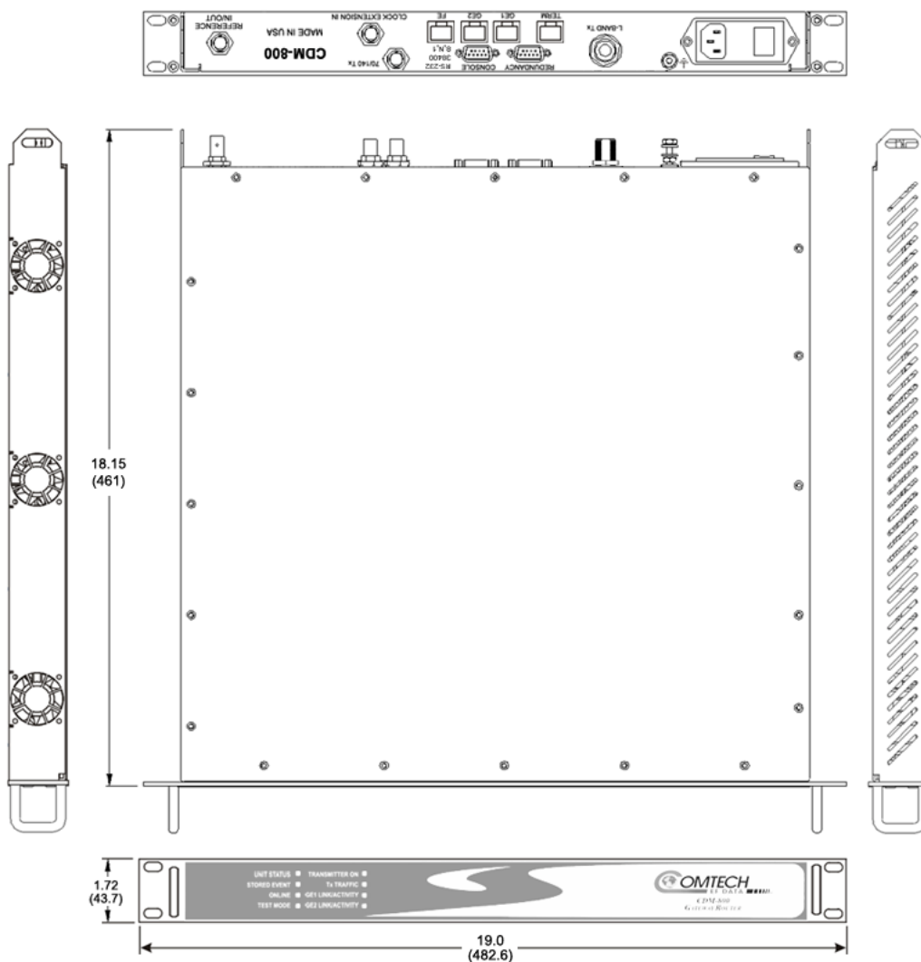
Figure 1-3. CDM-800 Dimensional Envelope
