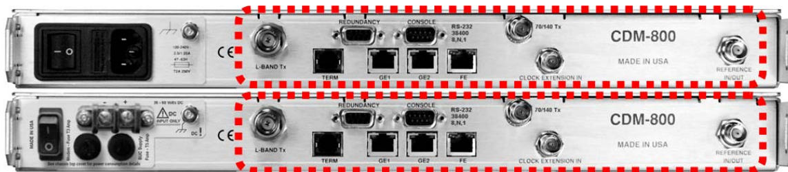
Figure 3-3. CDM-800 Cabling Connections
