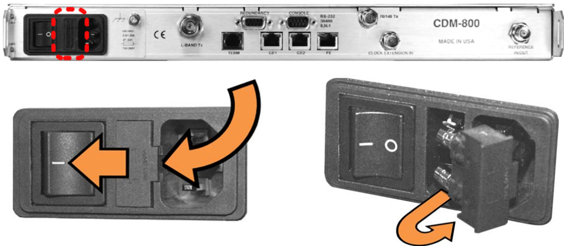
Figure 3-7. Replacing CDM-800 AC Fuses
