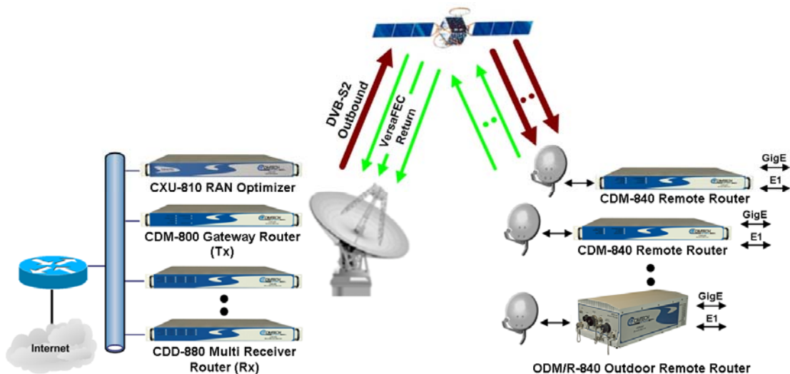
Figure 1-2. Advanced VSAT Series Network Topology Example
