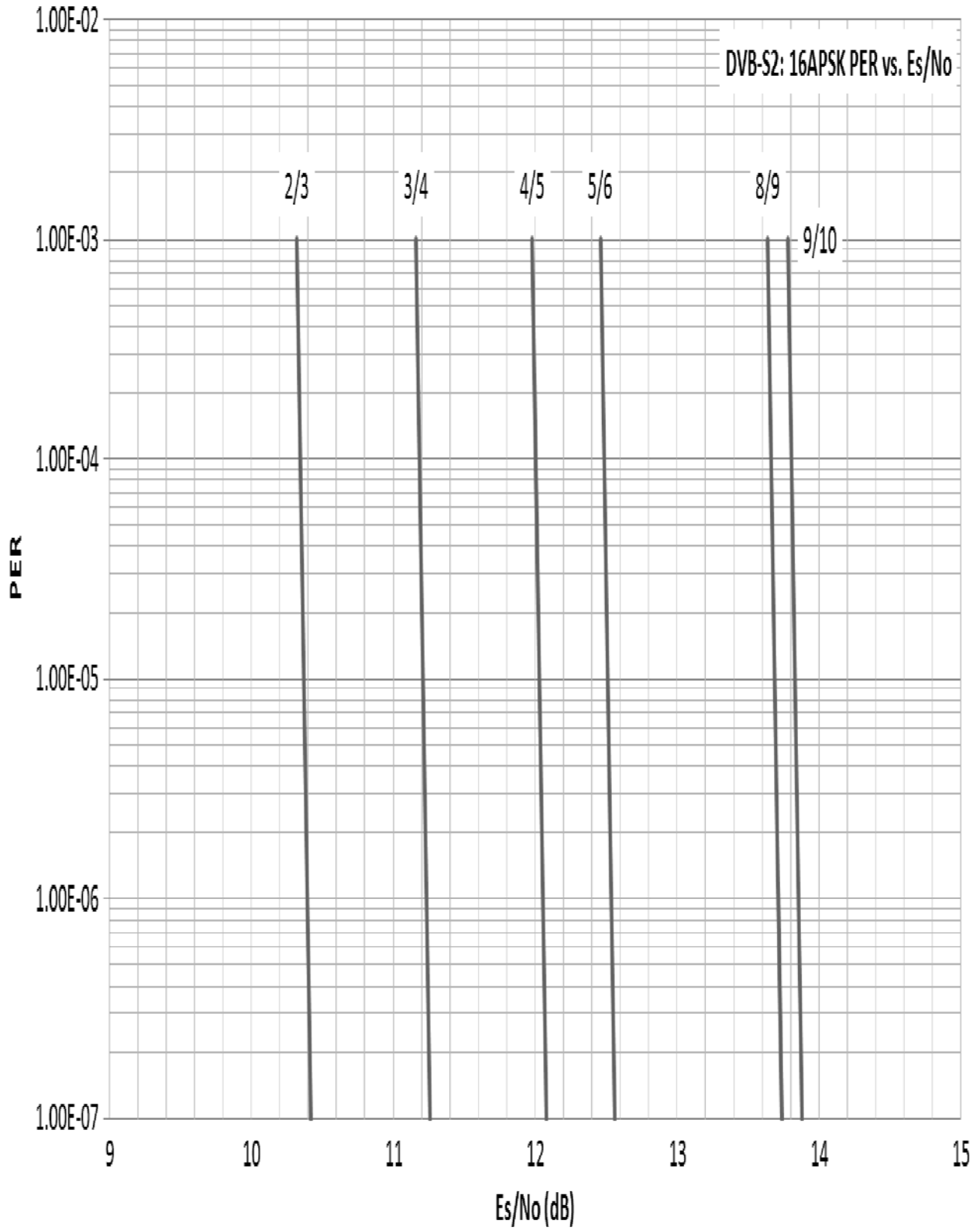
Figure B-3. DVB-S2 16APSK Packet Error Rate versus Es/No
