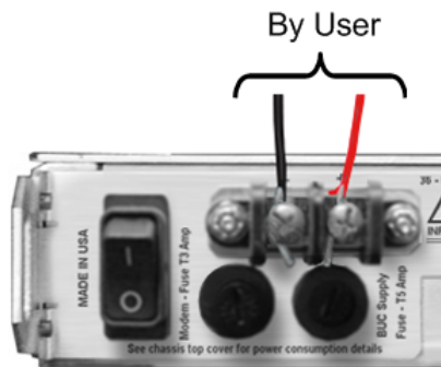
Figure 3-9. Applying DC Power to the CDM-800
