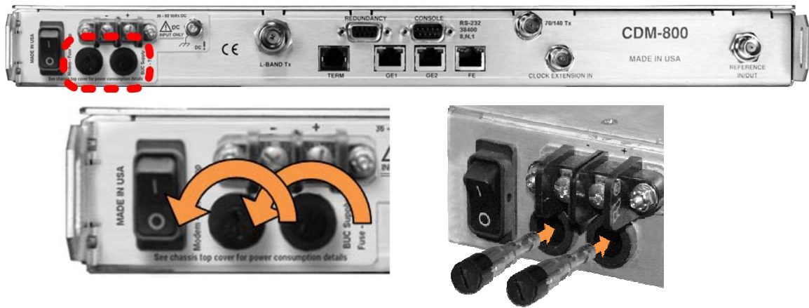
Figure 3-10. Replacing CDM-800 DC Fuses
